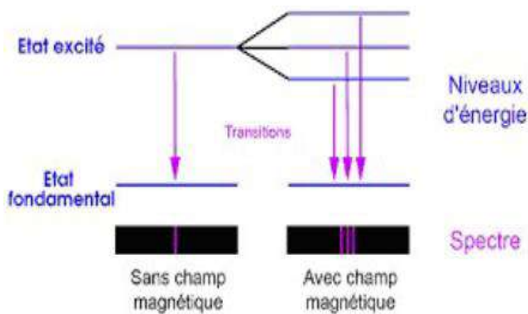
Figure 13 : effet Zeeman
